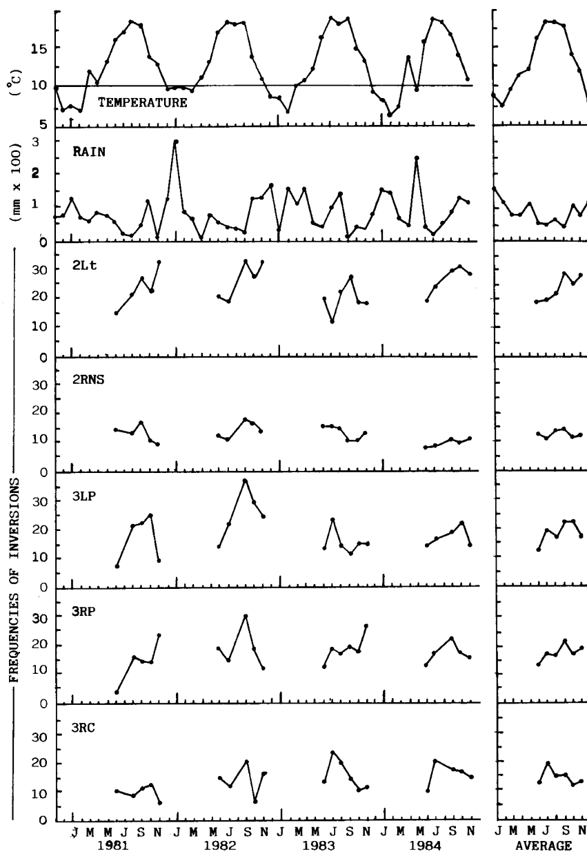
Fig 1. Four-year data of the average monthly temperature and rainfall, and frequency of the inversions.
