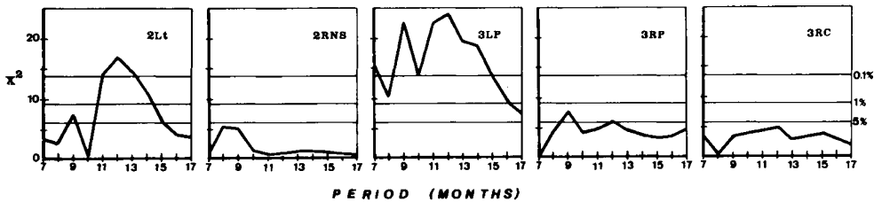
Fig 2. Periodicity testing charts for the 5 inversions. Horizontal lines mark the critical \chi^2 values for 3 significance levels.
