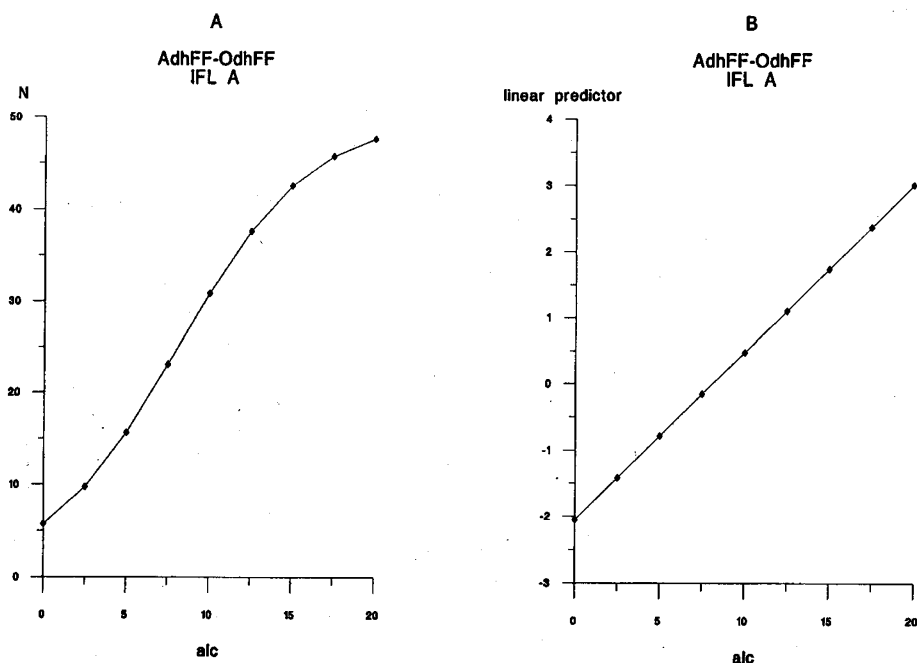
Figure 2. Predicted number of dead pupae (A:N) and values of the linear predictor (B) for the Adh^{FF}-Odh^{FF} strain constructed from IFL A on the basis of the strain model. A) ISR = (50 - N_0)/50 where N_0 is the number of dead larvae at 0 % alcohol; LD_{50} is the alcohol concentration at N = 25 (50 % of the original number of larvae). B) Linear predictor \eta = \ln(p/q) where p is death rate, q is survival and p = 1 - q ; \eta = a + b.x where x is alcohol concentration; a is the intercept and b is the slope for the Adh^{FF}-Odh^{FF} strain constructed from IFL A: \eta = -2.05 + 0.253.x .
