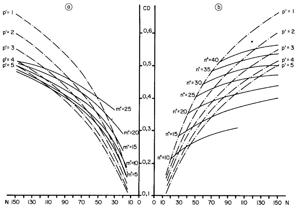
FIG. 1. — Coefficient of determination (CD) as a function of herd size ( N ), number of NS bulls ( p' ) and progeny numbers of the AI reference bull ( m ) and per NS bull ( n ) (respectively)
