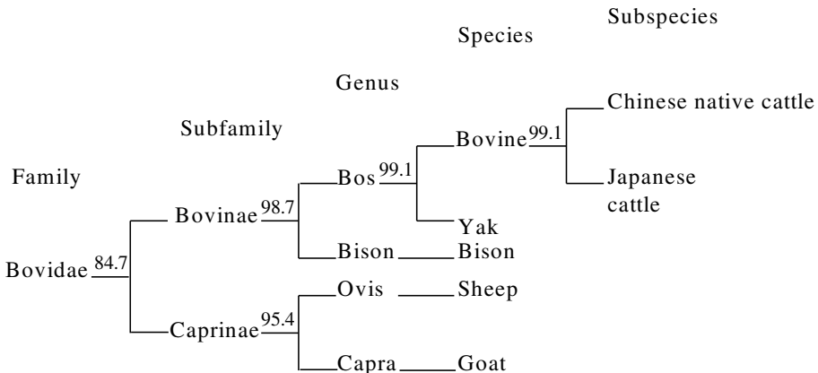
Figure 3. Evolutionary tree based on the amino acid identities among Bovidae SRY proteins. The numbers are percentage amino-acid identities.
