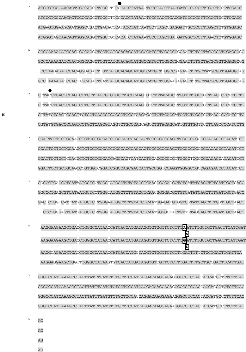
Figure 3. Conservation of nucleotide and amino-acid wild-type sequence of the horse, mouse and human exon 1 and exon 2 of the MATP gene. SNP6 and SNP7 positions are represented by dots (position 32 and 165 respectively in the nucleotide sequence). SNP8 position is represented by frames (position 457 in the nucleotide sequence, and position 153 in the amino-acid sequence). Identical residues are shaded. The first exon is 385 nucleotides long. (Accession numbers AY187092, AY187093).
