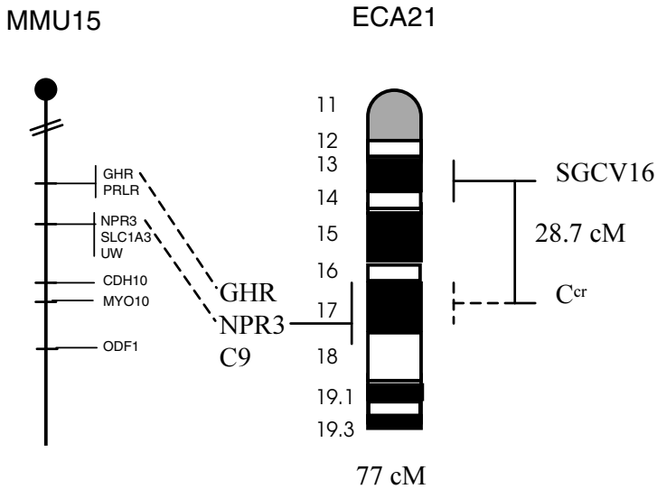
Figure 1. Distribution of markers around the underwhite locus on horse chromosome 21 and mouse chromosome 15.
