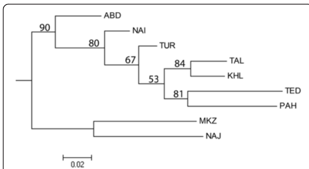
Figure 4 Neighbor-Joining tree based on D_A genetic distances for nine populations. Numbers at the nodes are bootstrap values based on 1000 permutations.
