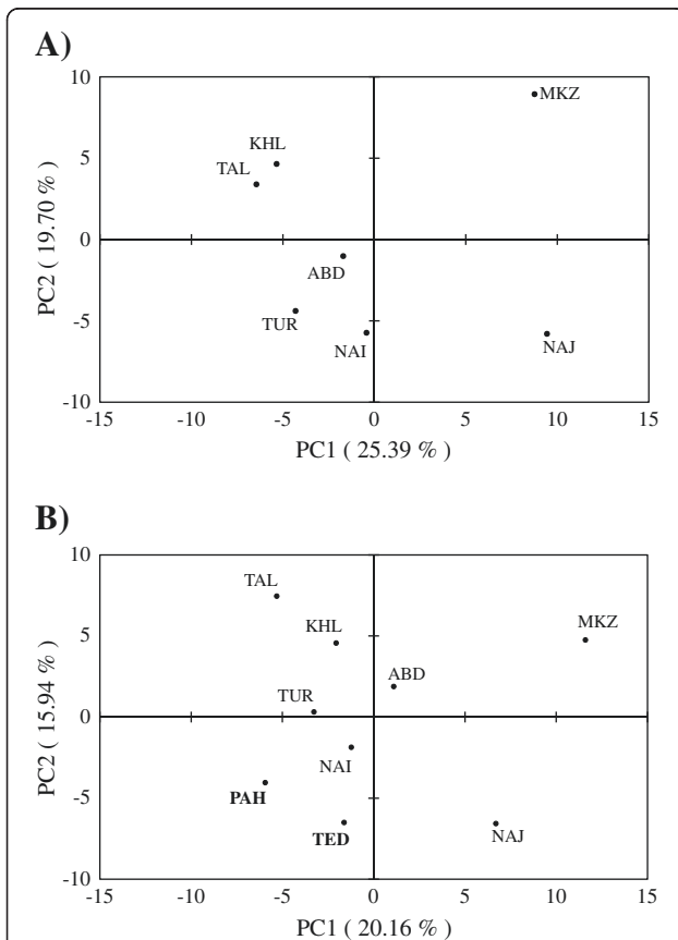
Figure 5 Principal component analysis. The principal components were extracted by correlation coefficients of Pearson, based on allele frequencies. A) PCA analysis of seven Iranian breeds. B) PCA analysis of nine goat breeds (Iran and Pakistan).
